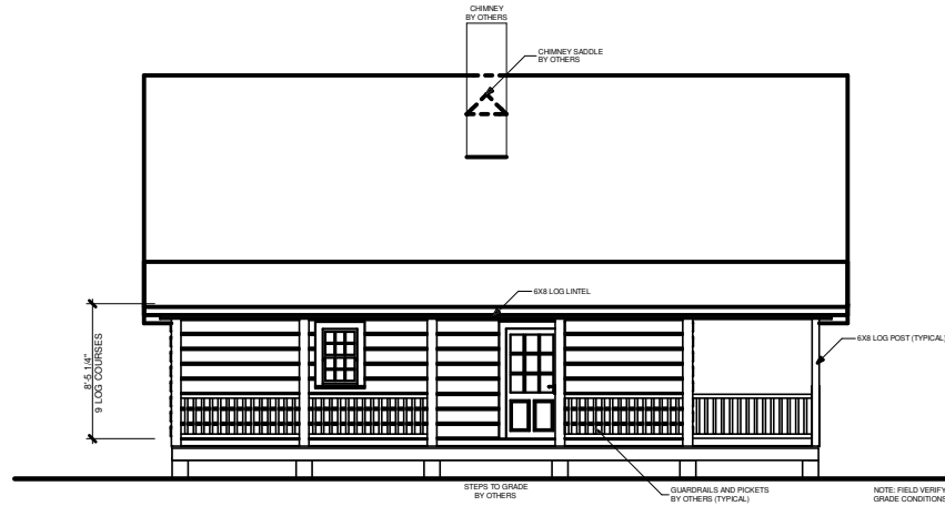
LEFT ELEVATION
