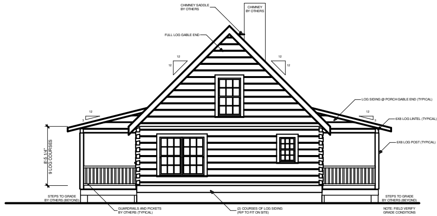
REAR ELEVATION
