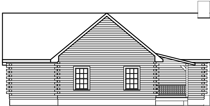
REAR ELEVATION
